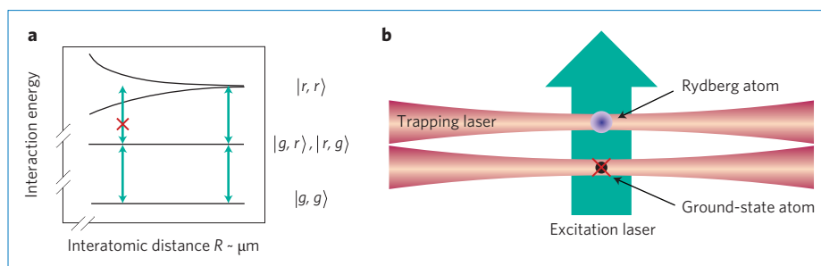
Figure 1 | Rydberg dipole blockade. a , Two atoms in a Rydberg state ( |r\rangle ) interact via dipolar forces over distances of several micrometres, whereas the interaction involving atoms in the ground state ( |g\rangle ) is negligible. Either atom can be excited by a resonant laser field, but not both atoms simultaneously, if the interaction-induced energy shift is larger than the width of the resonance line. b , In the experiments of Urban et al. 1 and Gaëtan et al. 2 , two single atoms are held in independent optical dipole traps formed by the foci of two far-detuned laser beams. The distance between the atoms can be adjusted down to a few microns. The atoms are illuminated by a resonant laser field exciting them to Rydberg states.
