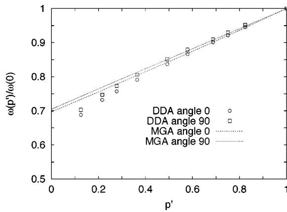
FIG. 2. Calculated surface plasmon frequencies \omega_{0,\parallel}(p')/\omega_0 and \omega_{0,\perp}(p')/\omega_0 , corresponding to incident light polarized parallel and perpendicular to the NLC director, for metal nanoparticles coated with NLC and embedded in an air host, plotted as a function of volume fraction p' of the coated particle which is composed of metal. The coating is assumed to be the NLC E7, which has indices of refraction n_{\parallel}=1.75 , n_{\perp}=1.52 . The metal particles are taken to have the Drude dielectric function, and \omega_0=\omega_0(p'=1)=\omega_p/\sqrt{3} . Full and dashed lines: MGA; squares and circles: DDA.
