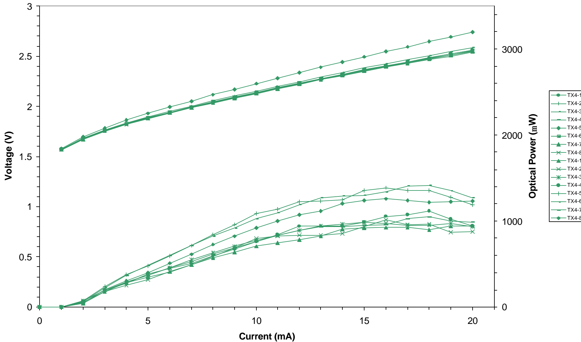
Second Batch of Oxide High Power VCSEL TX4 Current vs. Forward Voltage and Optical Power
