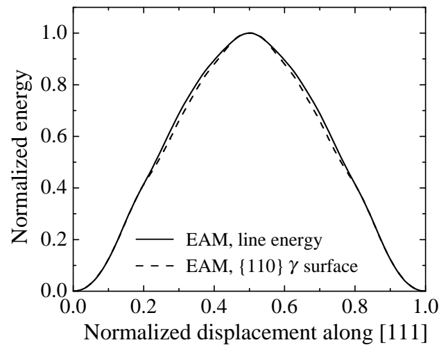
Figure 2: Normalized line and gamma surface energies.
