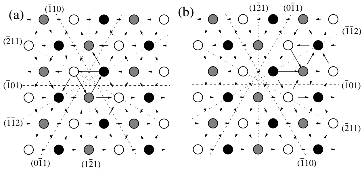
Figure 3: Motion of screw dislocation under stress.
