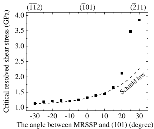
Figure 4: Critical resolved shear stress. The experimental Peierls stress is 415 MPa for 25°
