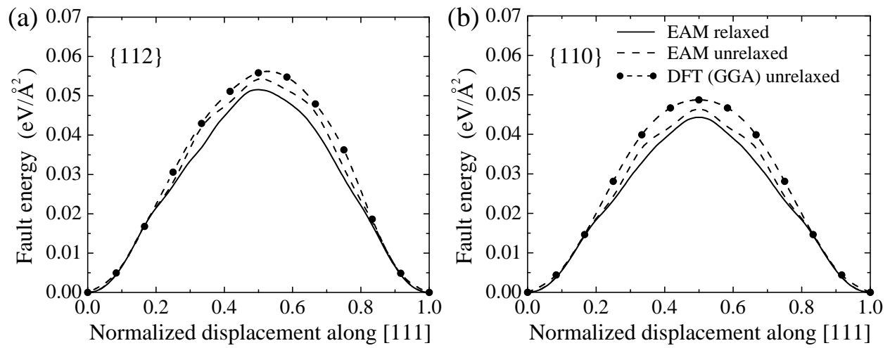
Figure 1: Gamma surfaces.
