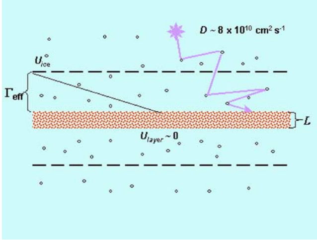
Figure 2. Photons created over the ice core are scattered by gas bubbles, diffusing (photon densities: U_{ice} \gg U_{layer} ) across depletion zones (thickness \Gamma_{eff} ) towards the contaminated layer (thickness L ), where they become absorbed by strongly chromophoric impurities.
