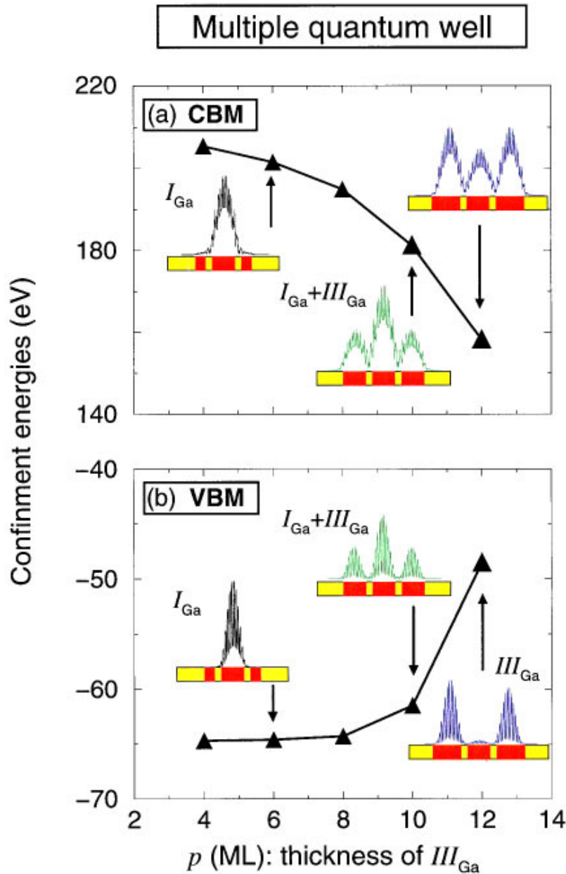
FIG. 2. (Color). Confinement energies (triangles) and wave-function amplitudes (insets) of the (a) CBM and (b) VBM of linear multiple quantum wells, as a function of the thickness p(III_{Ga}) of the outer GaAs layer. Other thicknesses are fixed at m(I_{Ga})=5 ML, n(II_{Al})=4 ML and q(IV_{Al})=8 ML. Red (yellow) denotes a GaAs (AlAs) layer.
