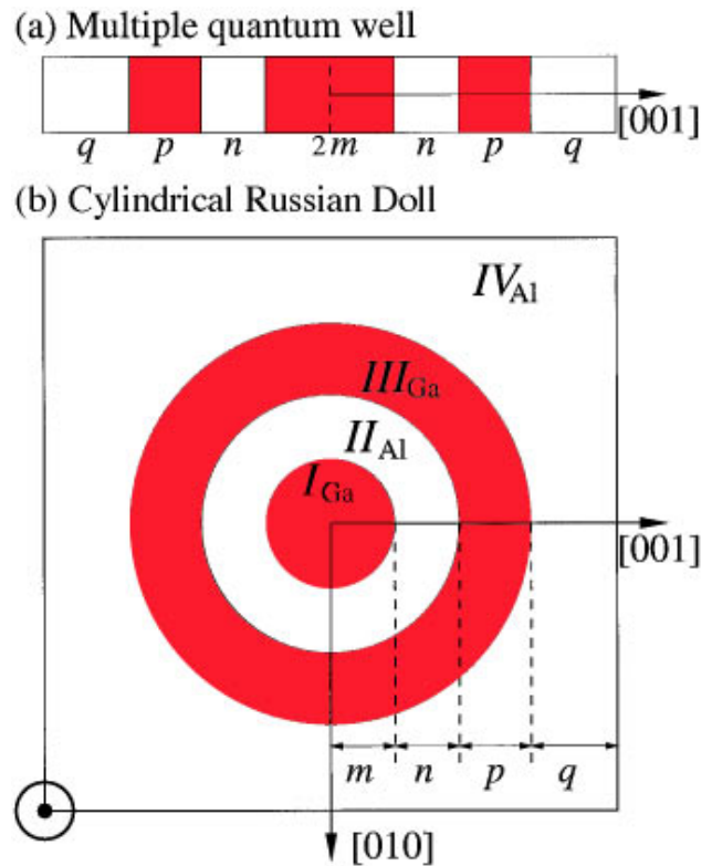
FIG. 1. (Color). Schematics of structure of (a) (001) multiple quantum wells, and (b) a {100} cross-section of an equivalent nested cylinder. These structures are made of alternating GaAs (red) and AlAs segments with thicknesses m , n , p , and q monolayers, respectively, in the order (starting from the center) I_{\text{Ga}} \rightarrow II_{\text{Al}} \rightarrow III_{\text{Ga}} \rightarrow IV_{\text{Al}} .
