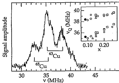
FIG. 3. The copper NQR spectrum (composed of ^{63}\text{Cu} and ^{65}\text{Cu} signals as indicated) from the metallic phase of oxygen-annealed \text{La}_2\text{CuO}_{4+\delta} (AF spectrum appears at \sim 100 MHz). This spectrum is nearly identical to that observed in \text{La}_{2-x}\text{Sr}_x\text{CuO}_4 ; the x dependences of the two NQR frequencies shown in the inset demonstrate this. The data for \text{La}_{2-x}\text{Sr}_x\text{CuO}_4 from Refs. [19-22] are represented with open symbols: circles [19], triangles [20], diamonds [21], and squares [22]. The values for the oxygen doped material (present work) are plotted as closed circles at the value of x (0.09) which produces an equivalent level of hole doping of the planes [12].
