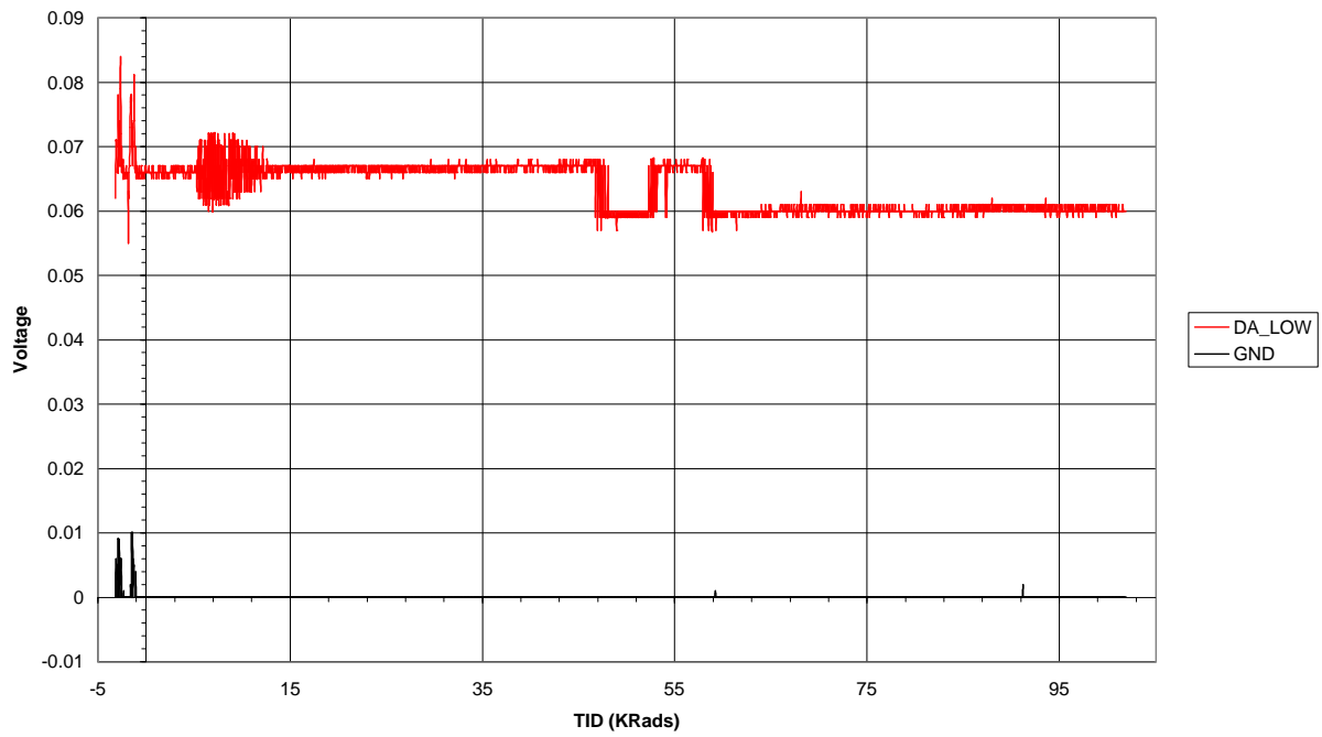
Cobalt 60: Diode Array (Low)
