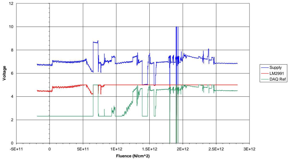
Reactor Neutrons + Photons: LM2991
