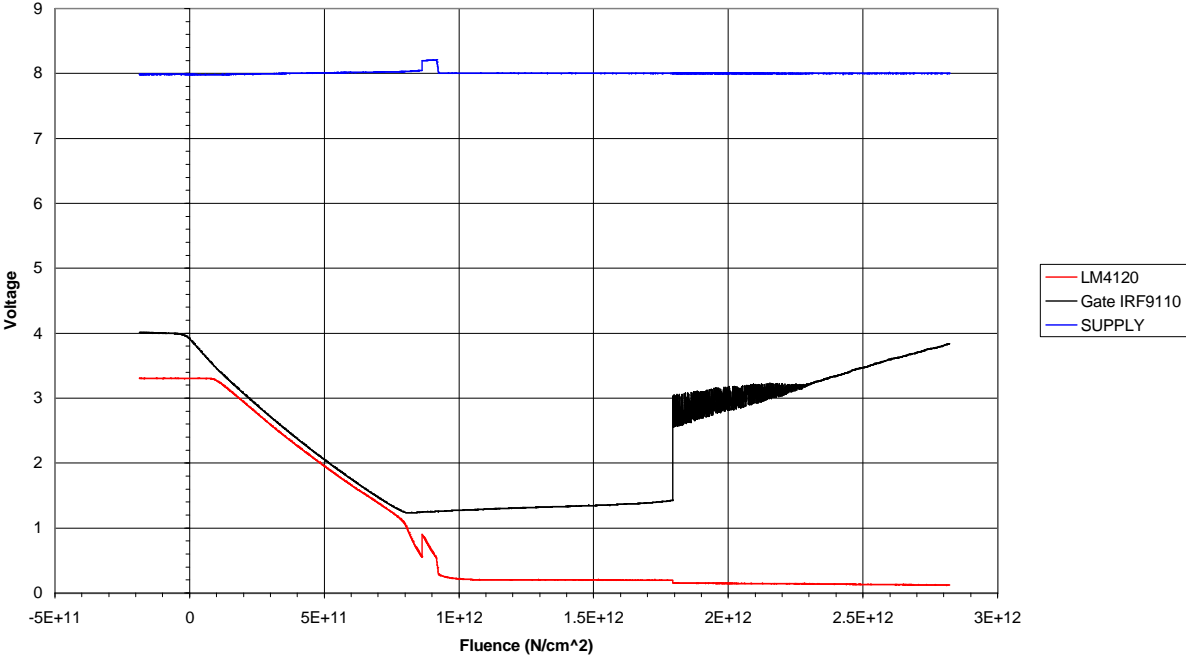
Reactor Neutrons + Photons: LM4120 and Pass Transistor
