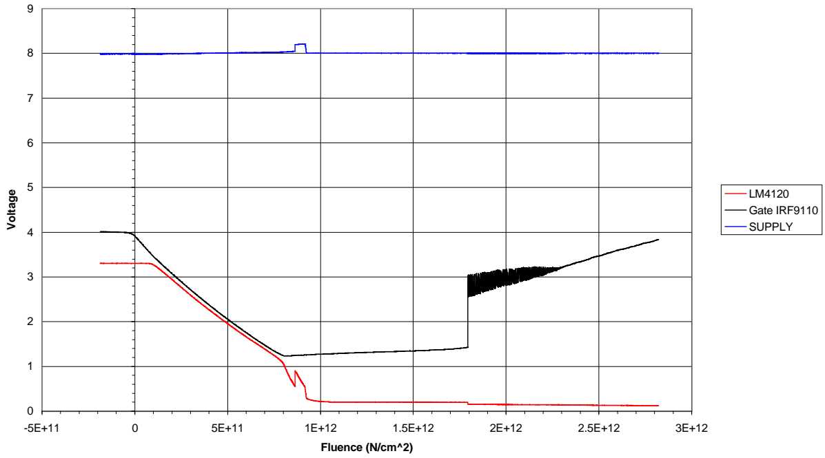
Reactor Neutrons + Photons: LM4120 and Pass Transistor
