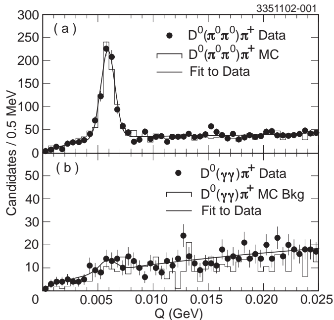
FIG. 1: The Q distributions for D^{*+} \rightarrow D^0 \pi^+ where D^0 \rightarrow \pi^0 \pi^0 (a) and D^0 \rightarrow \gamma \gamma (b). The circles are from data and the solid curves are the fit to the data. The histograms are from the normalized Monte Carlo expectations.
