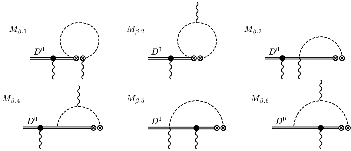
Figure 5: The diagrams which give nonzero amplitudes with one \beta -like coupling.
