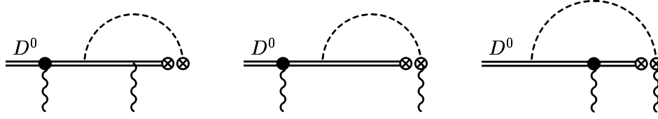
Figure 4: The diagrams with one \beta -like (14) coupling (described by \bullet ), which give vanishing amplitudes.
