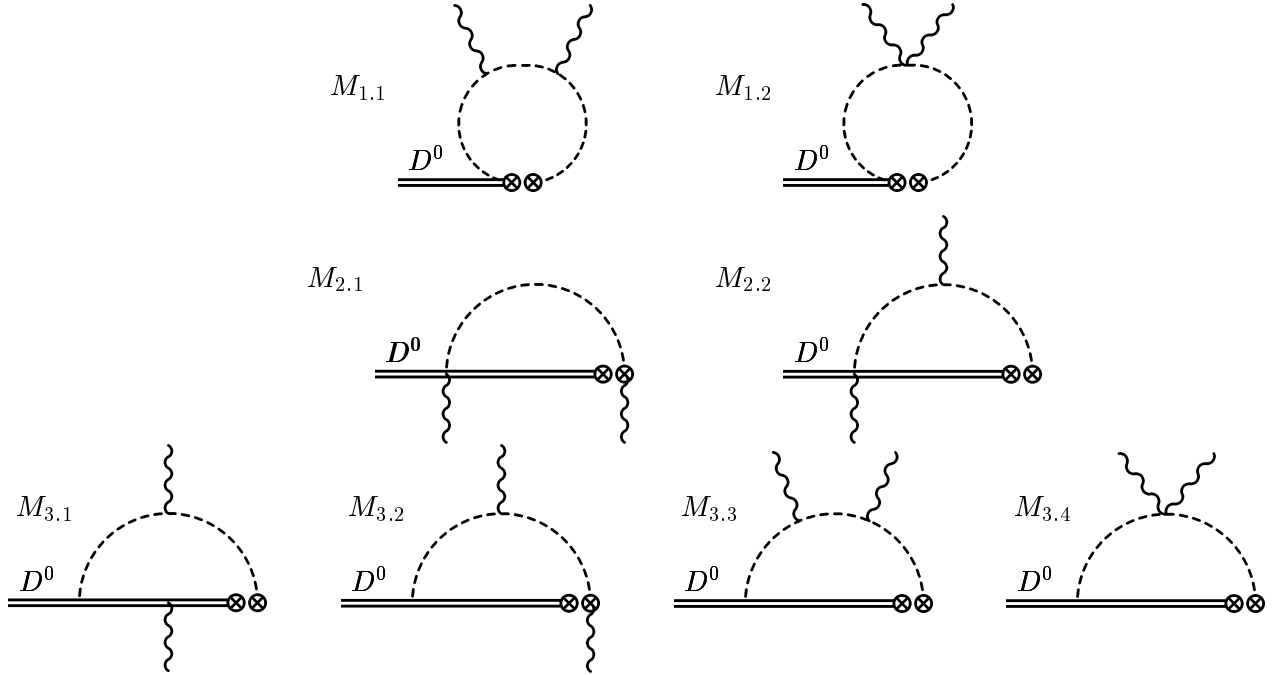
Figure 2: One loop diagrams, not containing beta-like terms (14), that give nonvanishing contributions to the D^0 \rightarrow \gamma\gamma decay amplitude. Each sum of the amplitudes on diagrams in one row M_i = \sum_j M_{i,j} is gauge invariant and finite. Numerical values are listed in Table 1.
