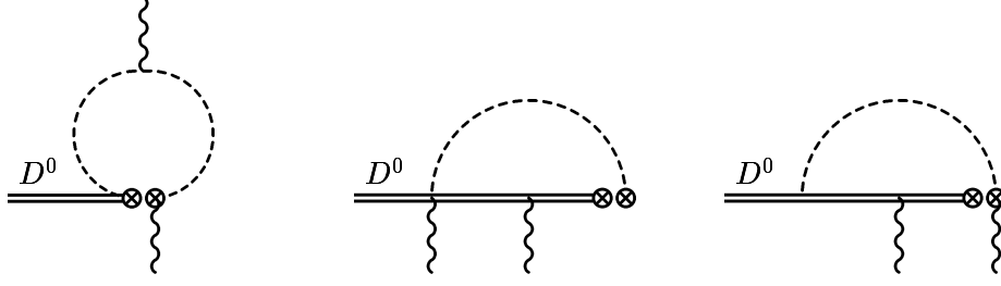
Figure 1: One loop diagrams (not containing \beta -like terms (14)) that give vanishing contributions. The dashed line represents charged Goldstone bosons flowing in the loop ( K^+ , \pi^+ ), while the double line represents heavy mesons, D and D^* .
